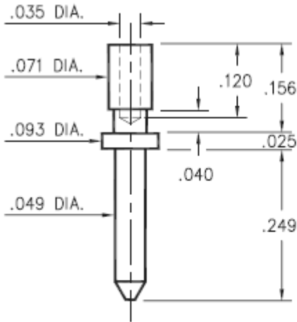
3139-0-00-XX-00-00-08-0 Wire Termination
